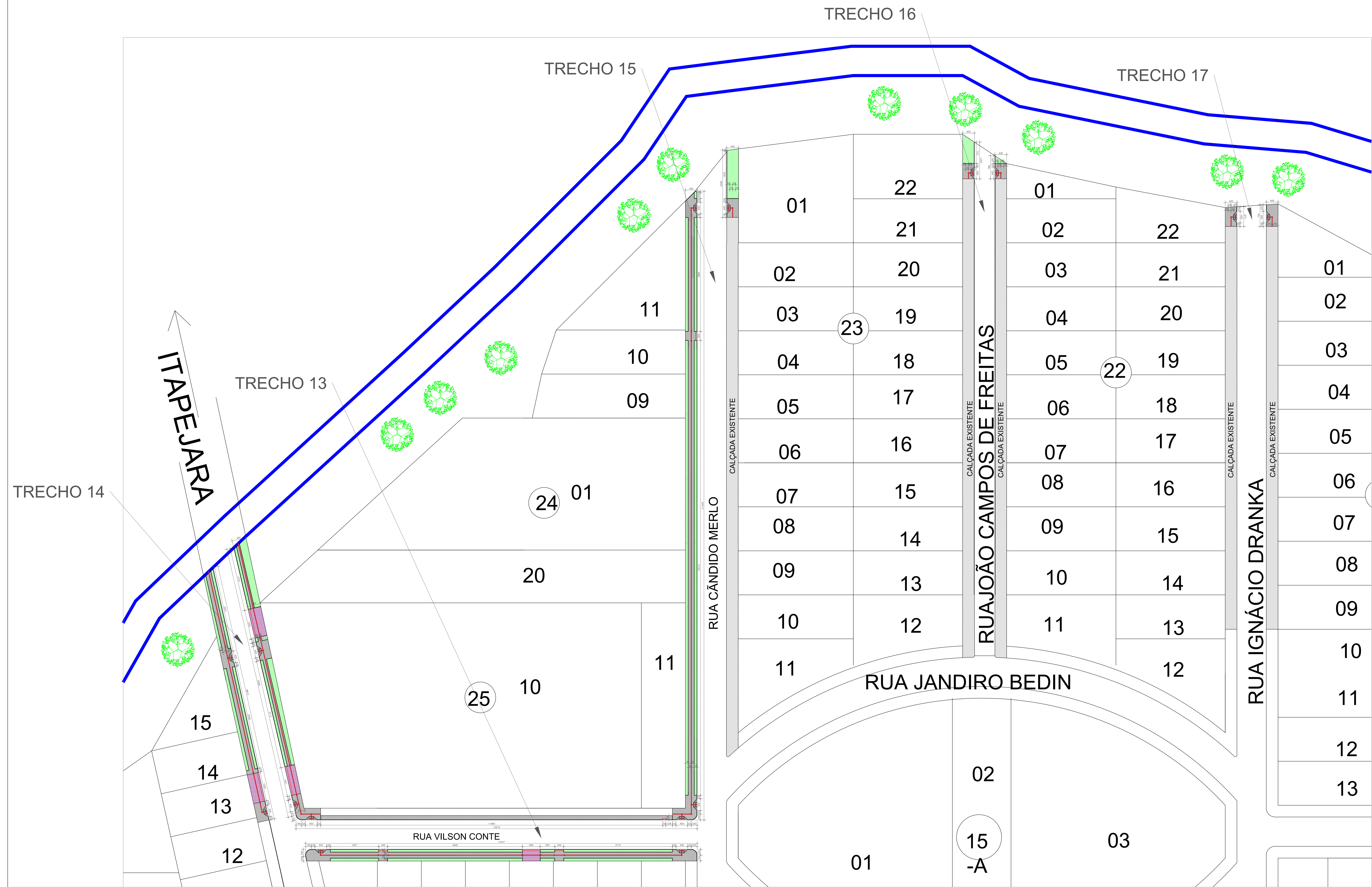
TRECHOS 13, 14, 15, 16 E 17 ESCALA 1/400
